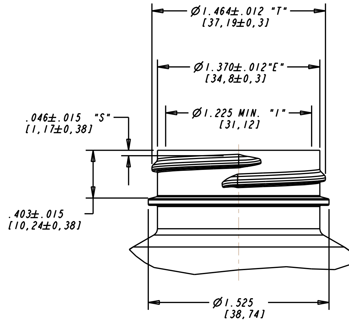
DETAIL A M38-400 NECK FINISH 6 T.P.I., 1 THREAD TURN .250 MIN. "I" DEPTH SCALE 2.000
