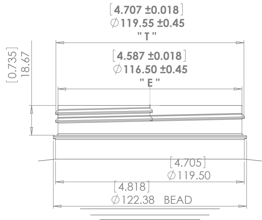
DETAIL A SCALE 2 : 3
